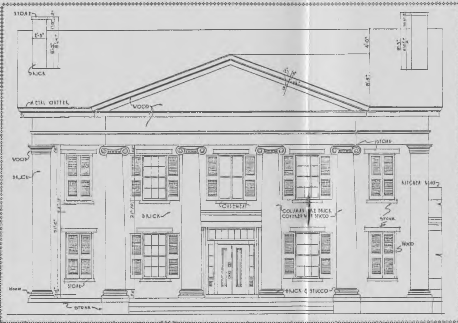
Front elevation of the BIBB house drawn in 1834 by Wilfred Van Valkenburgh for HABS. Representative of Greek Revival styling are the massive proportions, symmetry of the facade, pedimented portico with two-story Ionic columns, corner pilasters, and entrance having a rectangular top-light and double doors each with a single full-length panel.
